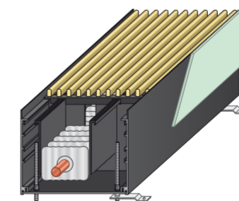
Trench heating system
